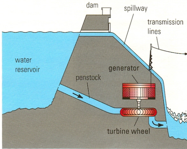
Cross section of a dam
